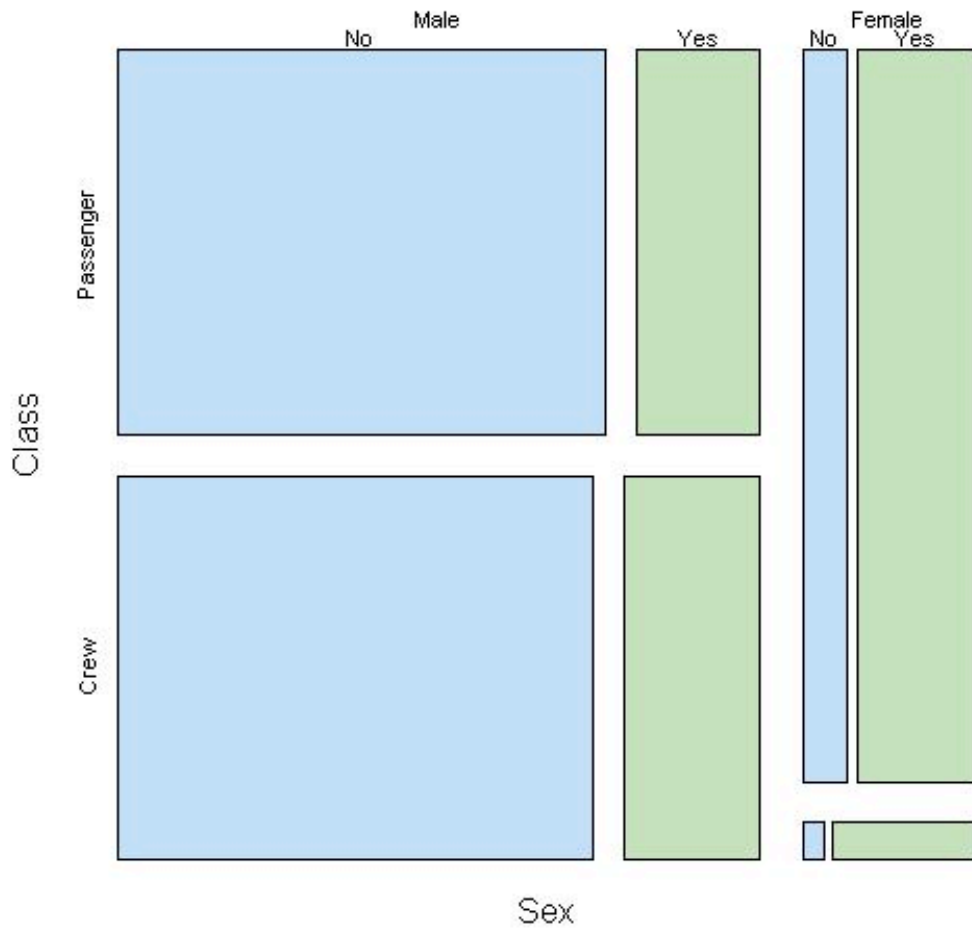
Titanic Mosaic Survived over Class & Sex
